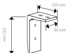
Montage mural consoles murales
