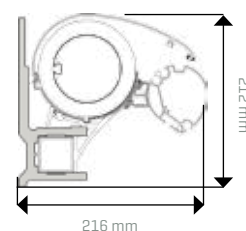
Montage mural consoles murales
